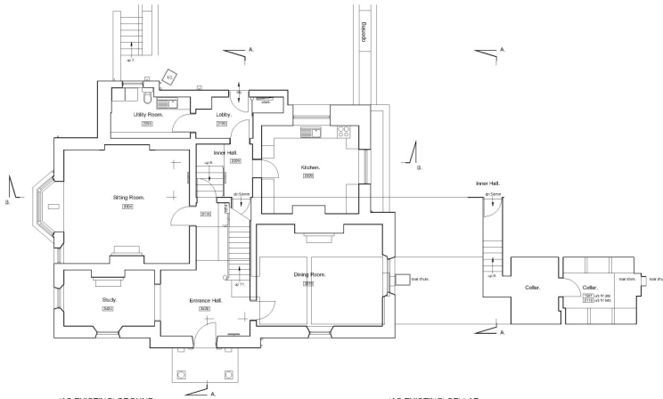
'AS EXISTING' GROUND FLOOR PLAN.
